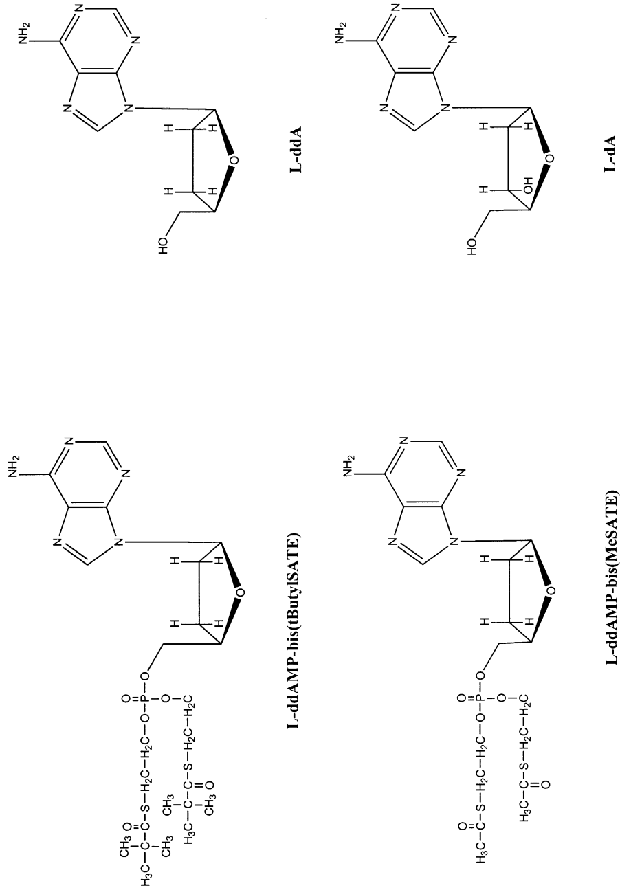
Fig. 1. Chemical structure of L-dA, L-ddA, L-ddAMP-bis(MeSATE) and L-ddAMP-bis (tButylSATE).
